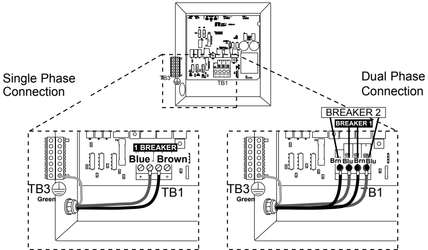
Figure E (Export 50 Hz 230 VAC Connection*)
